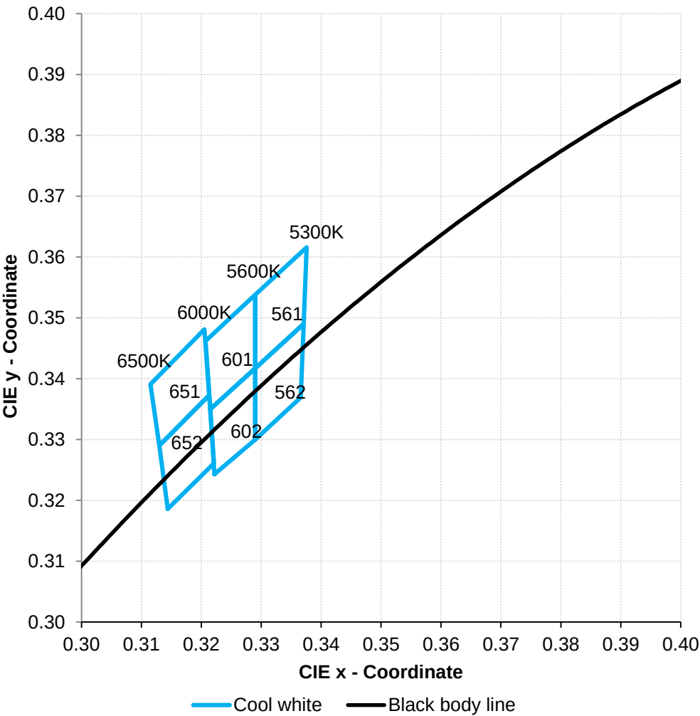
Chromaticity diagram:
