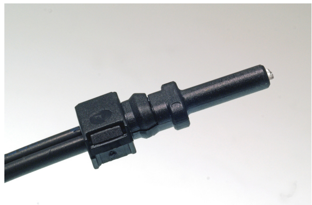
Figure 6 POF Cable with Closed AFBR-S10PS011Z Connector
