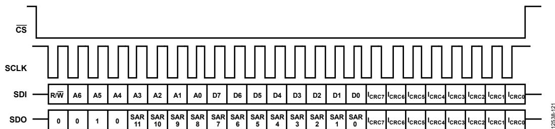
Figure 104. SAR ADC/Diagnostic Mode—CRC Enabled
