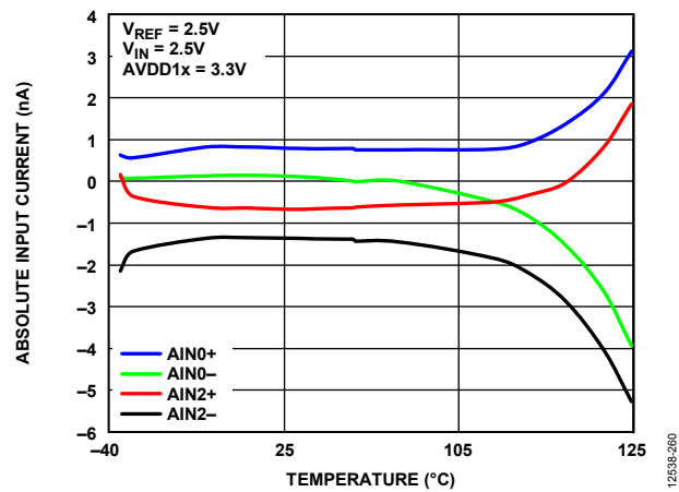
Figure 60. Absolute Input Current vs. Temperature, Low Power Mode
