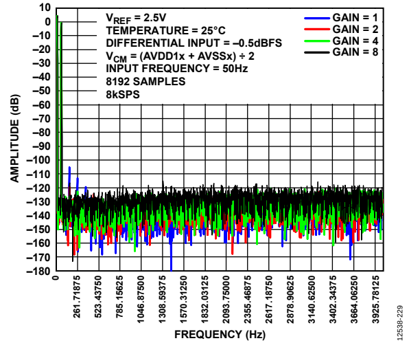
Figure 29. FFT at 8 kSPS, Low Power Mode, Input Frequency ( f_{IN} ) = 50 Hz
