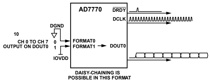
Figure 114. FORMATx Pin Configuration—FORMAT0 = 0, FORMAT1 = 1
