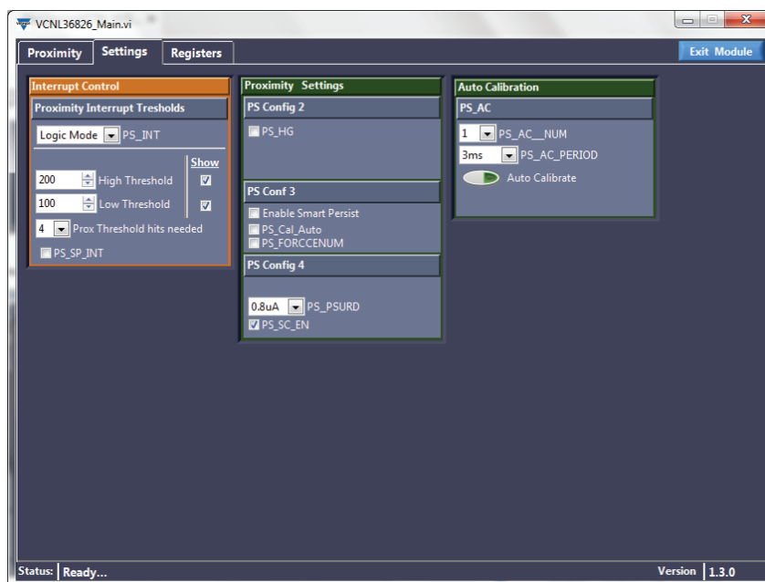
Fig. 34 - Logic Mode
