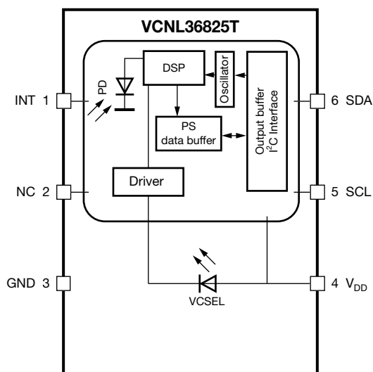
Fig. 3 - VCNL36825T Detailed Block Diagram
