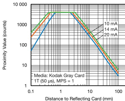
Fig. 15 - Proximity Value vs. Distance for 1T
