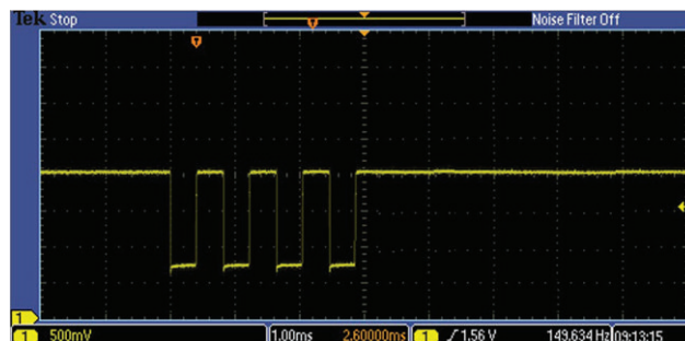
Fig. 40 - PS_IT = 8T (400 \mu s) and MPS = 4
