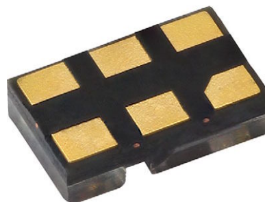
Fig. 2 - VCNL36825T Bottom View
