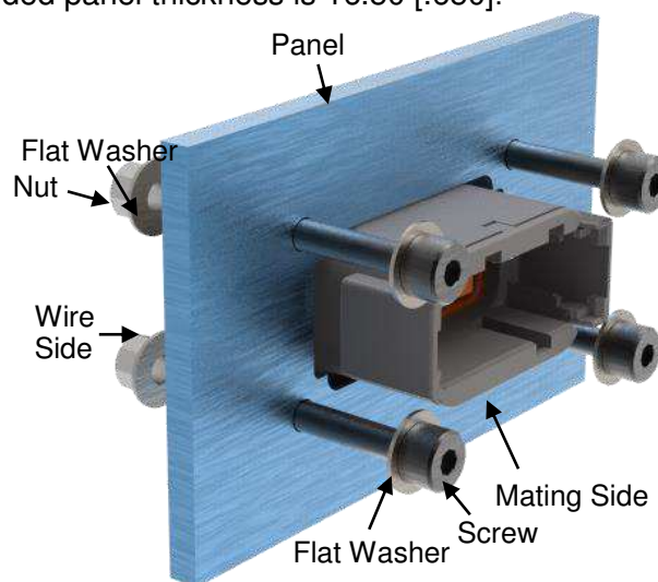
REAR MOUNT
