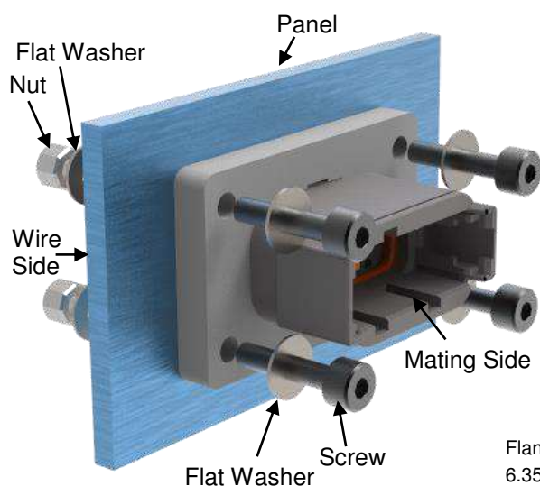
FRONT MOUNT
