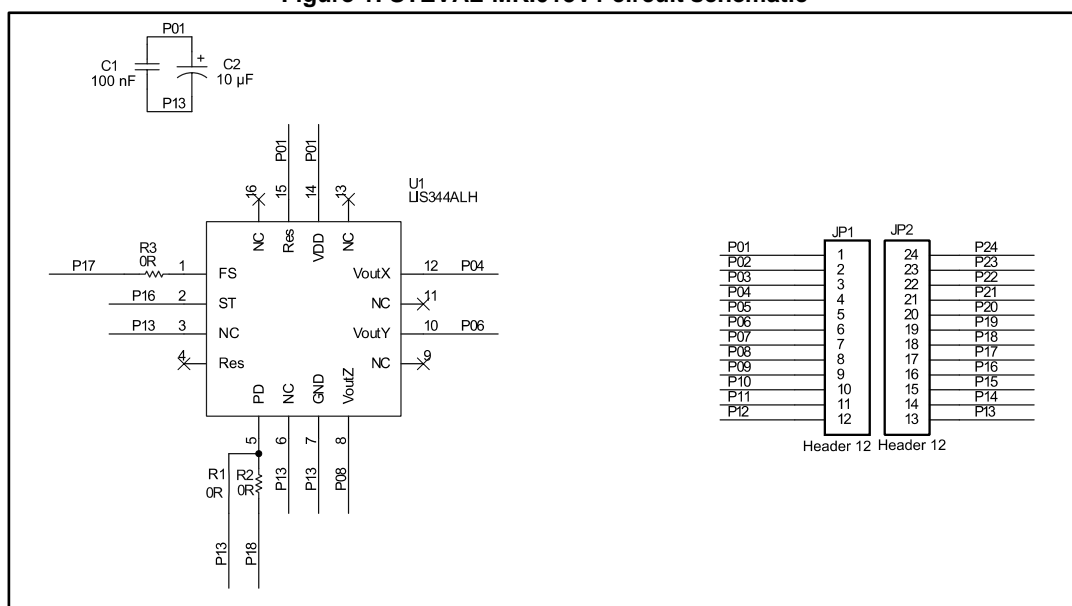
Figure 1: STEVAL-MKI015V1 circuit schematic
