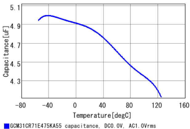
Tempeture Characteristics
