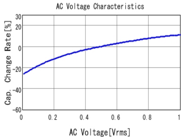
■ GRM32ER60J107ME20 C-AC Voltage capchange, DC0V, 25.0d
