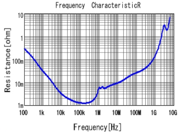
■ GRM32ER60J107ME20 R DC0V, 25degC
