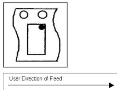
Figure 18. LGA-14 package orientation in carrier tape
