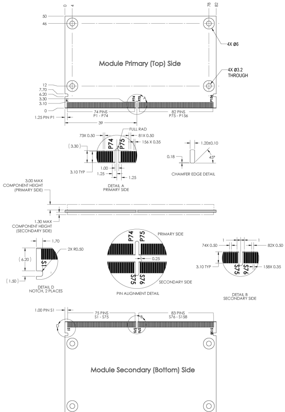
Figure 8 – iMX6SoloX COM Board Mechanical Outline
