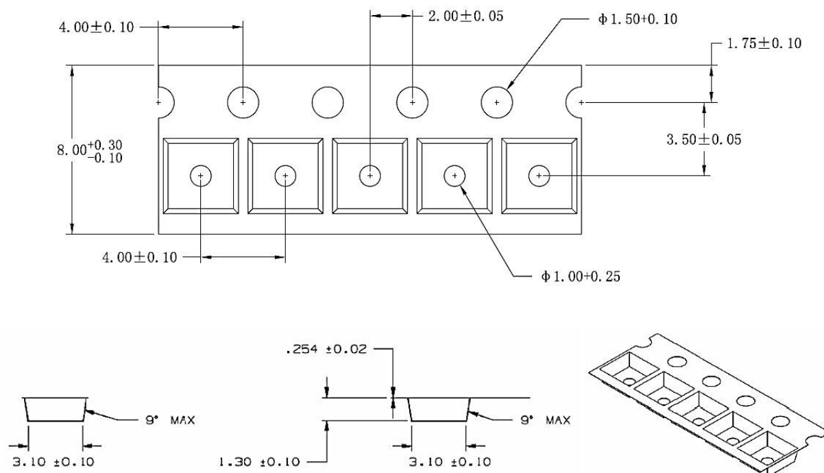
Figure 11.2 IQS128Tape Specification
