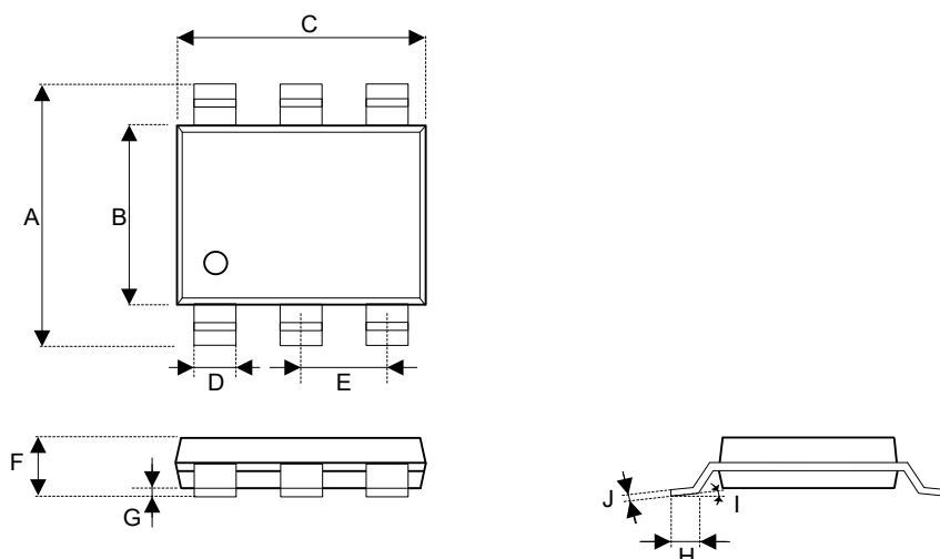
Figure 11.1 TSOT23-6 Packaging 6
