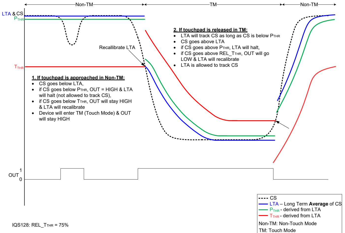
Figure 5.1 DYCAL Operation
