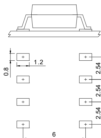
8-pin SOP
