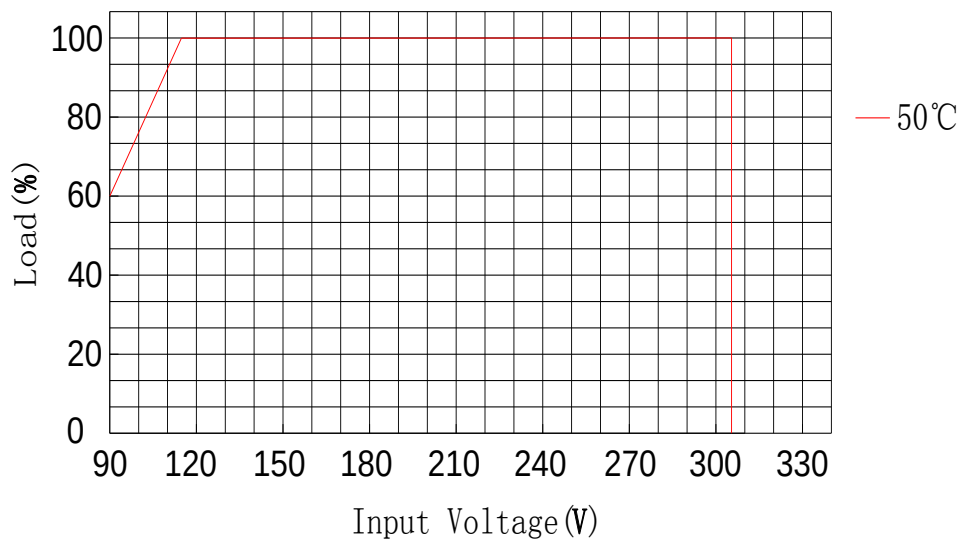
Input Voltage vs. Load Curve
