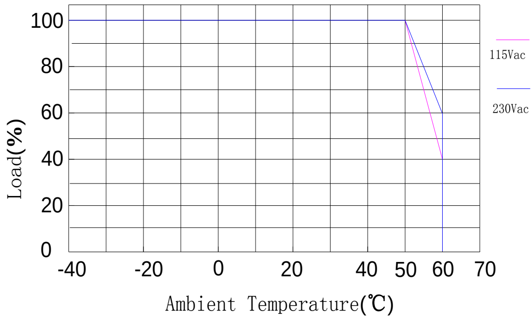
Temperature vs. Load Curve
