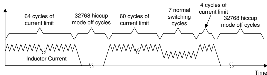
Figure 9-21. Hiccup Mode Overload Protection
