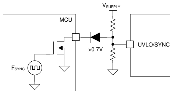
Figure 9-14. UVLO, Standby, and Clock Synchronization (a)
