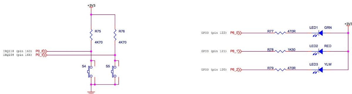
Figure 17: User buttons and LEDs
