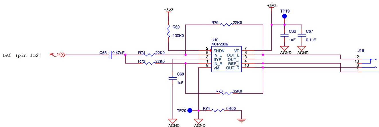
Figure 16: Audio output
