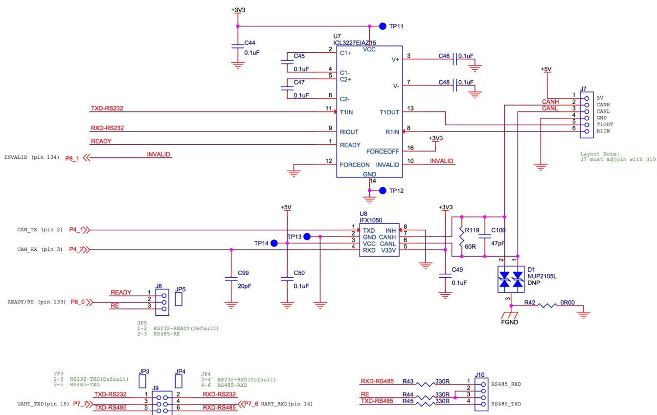
Figure 12: RS-232/485 and CAN interfaces
