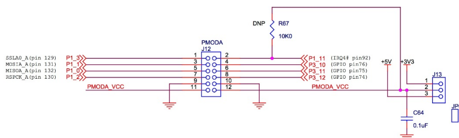
Figure 10: PMODA interface
