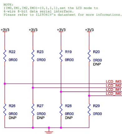
Figure 8: LCD interface mode selection
