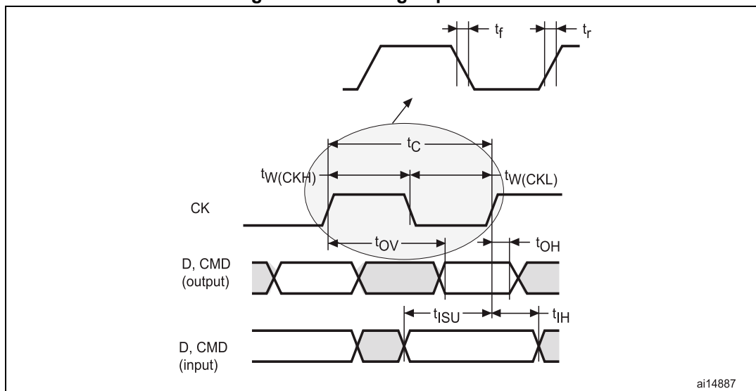
Figure 72. SD default mode
