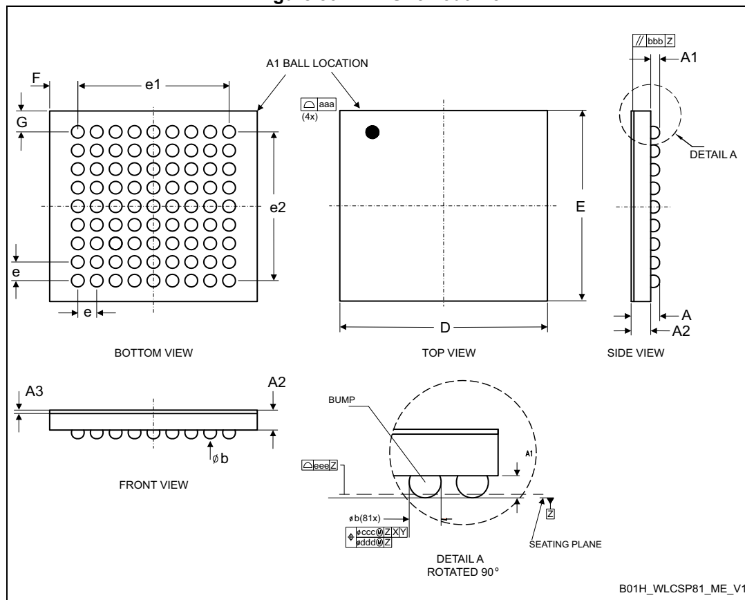
Figure 83. WLCSP81 outline
