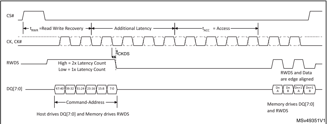
Figure 69. OCTOSPI HyperBus read with double latency
