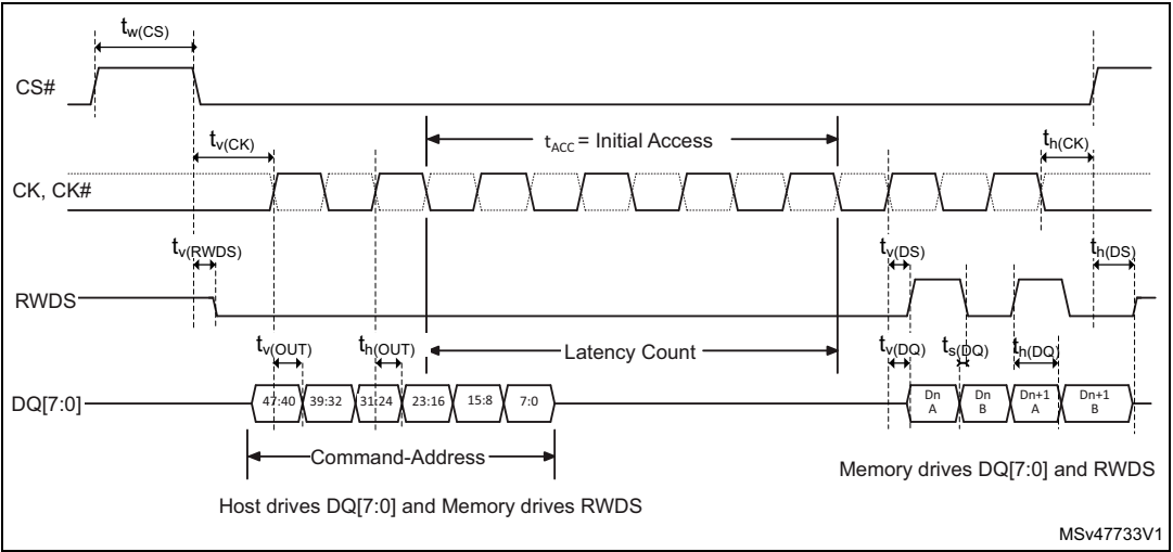
Figure 68. OCTOSPI HyperBus read
