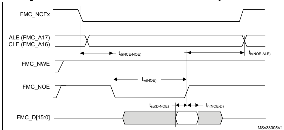
Figure 64. NAND controller waveforms for common memory write access
