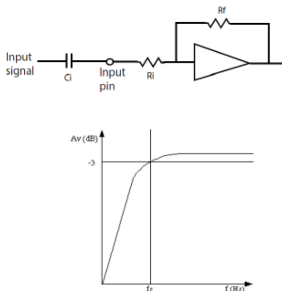
Figure 22. Input circuit and frequency response
