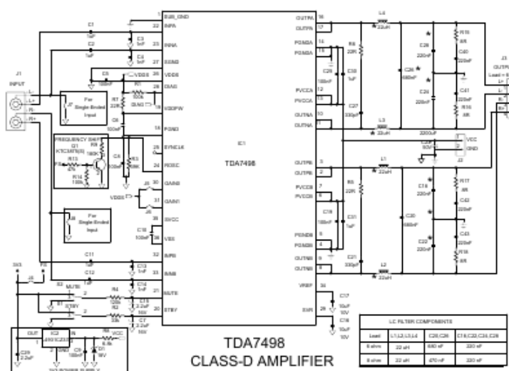
Figure 19. Application circuit for 6 \Omega or 8 \Omega speakers
