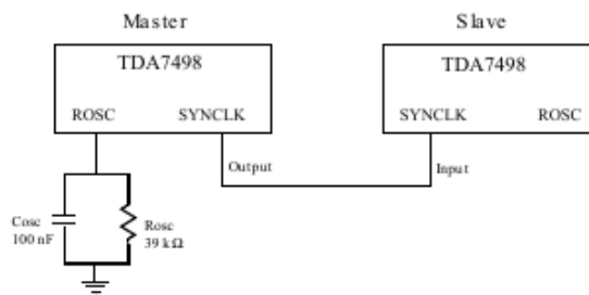
Figure 23. Master and slave connection
