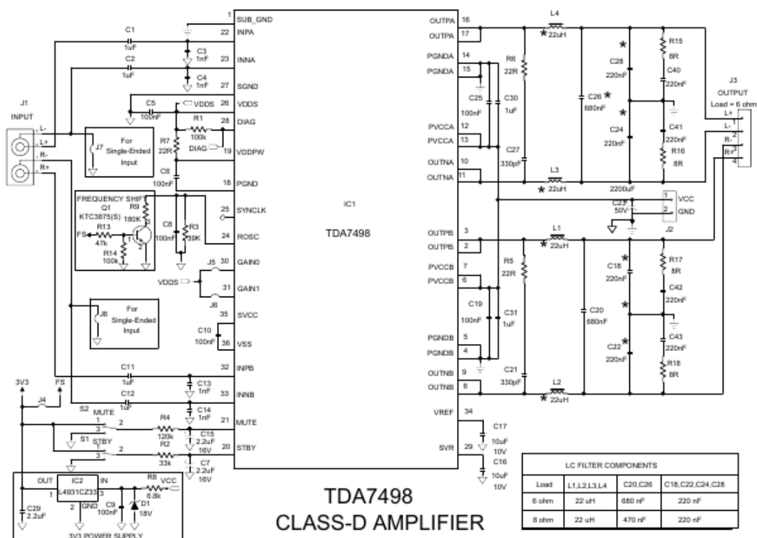
Figure 3. Test circuit for characterizations
