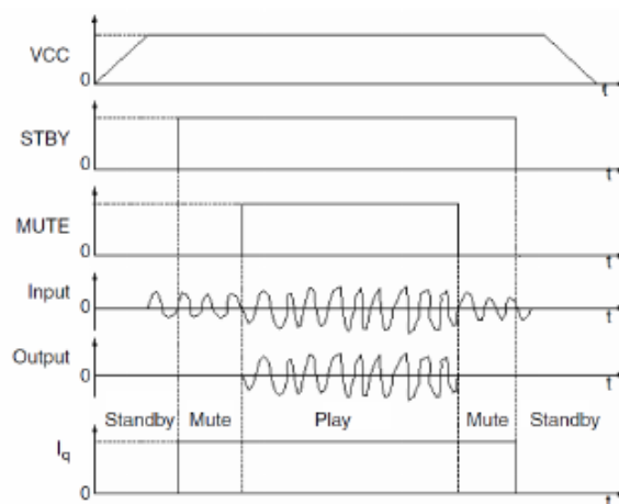
Figure 21. Turn on/off sequence for minimizing speaker "pop"
