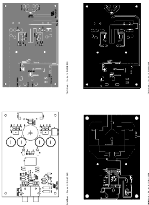
Figure 4. Test board
