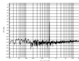
Figure 11. FFT performance (-60 dBFS)
