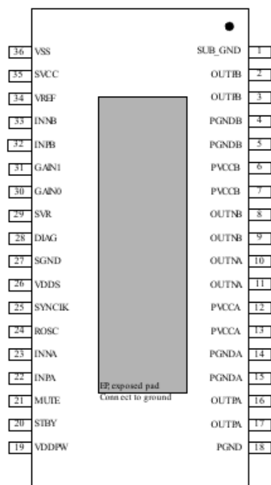
Figure 2. Pin connections (top view, PCB view)
