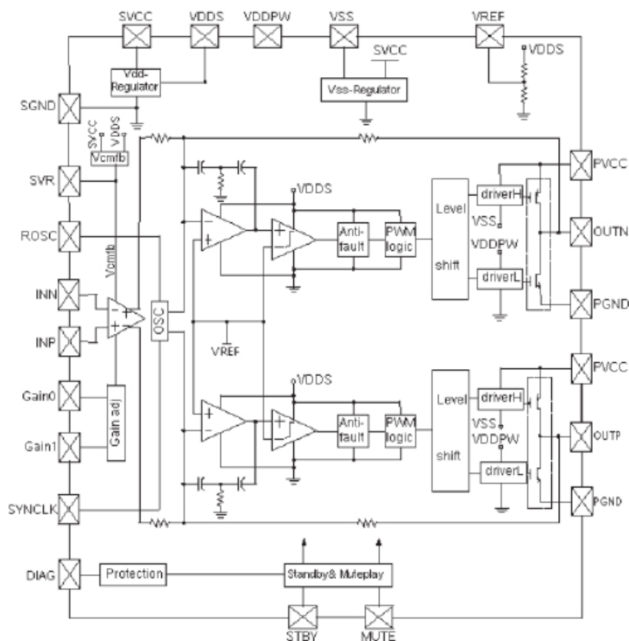
Figure 1. Internal block diagram (showing one channel only)
