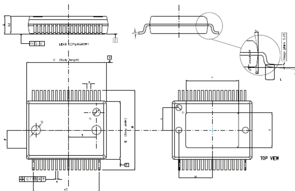
Figure 27. PowerSSO-36 EPU package outline
