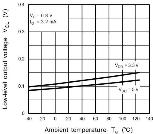
Fig. 12.2.4 V_{OL} - T_a
