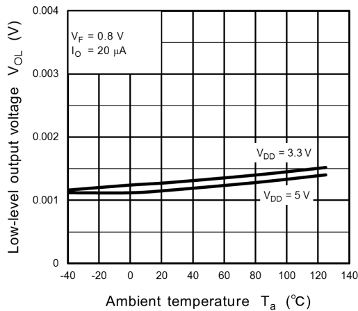
Fig. 12.2.3 V_{OL} - T_a
