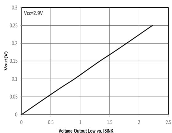
Figure 4 Voltage Output Low vs. ISINK (TPV809)
