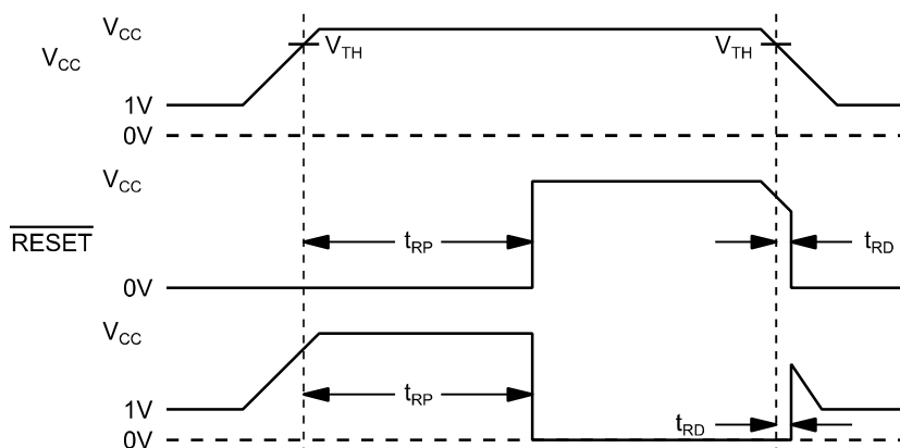
Figure 8 Reset Timing Diagram
