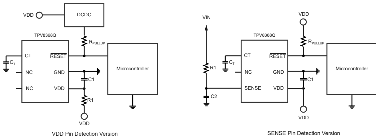
Figure 8. Typical Application Circuit
