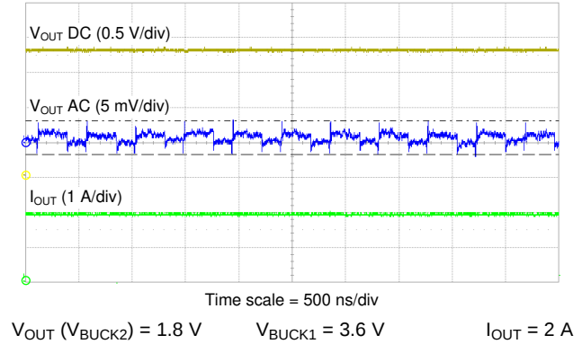
Figure 9-37. BUCK2 Output Voltage Ripple
