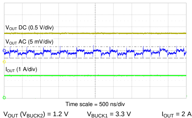
Figure 9-34. BUCK2 Output Voltage Ripple
