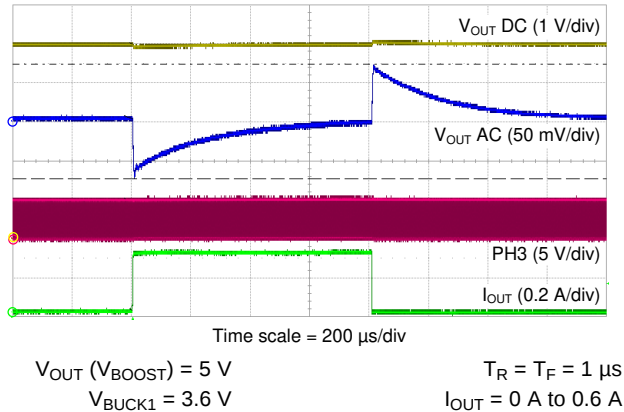
Figure 9-30. BOOST Load Transient
