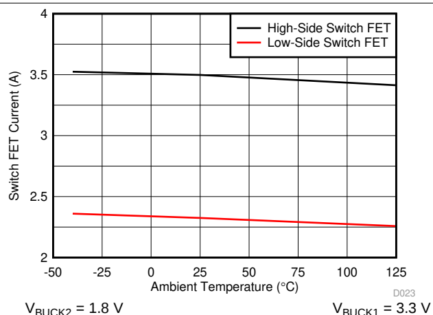
Figure 6-4. BUCK2 Current Limit ( I_{HS\_LIMIT\_BUCK2} and I_{LS\_LIMIT\_BUCK2} )
