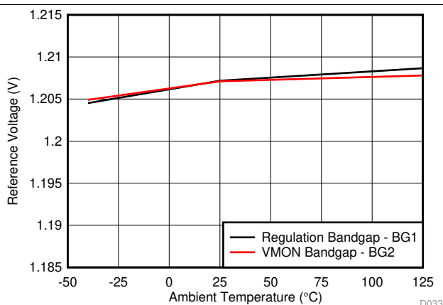
Figure 6-17. Regulation Bandgap (BG1) and Monitoring Bandgap (BG2)
