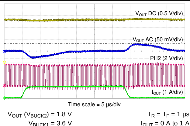
Figure 9-27. BUCK2 Load Transient
