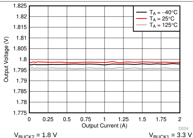
Figure 6-9. BUCK2 Output Voltage
