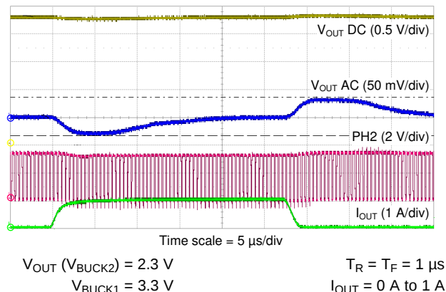
Figure 9-25. BUCK2 Load Transient
