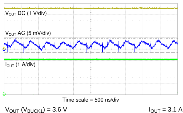
Figure 9-32. BUCK1 Output Voltage Ripple
