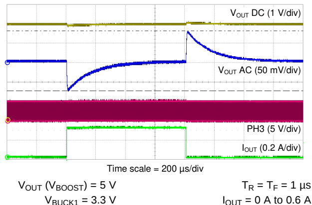
Figure 9-29. BOOST Load Transient
