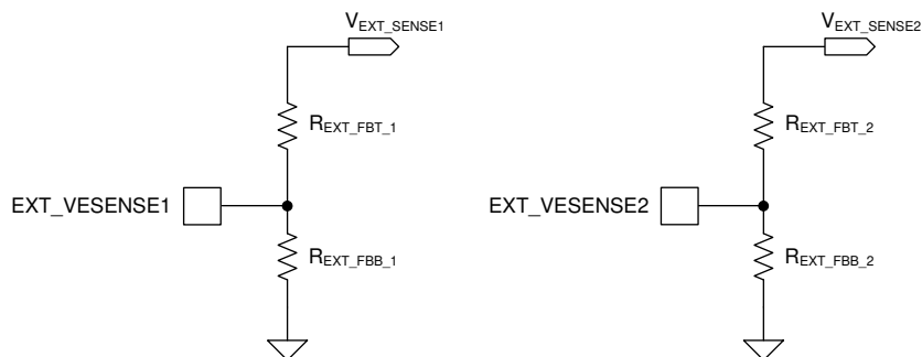
Figure 8-31. External VSENSEx
