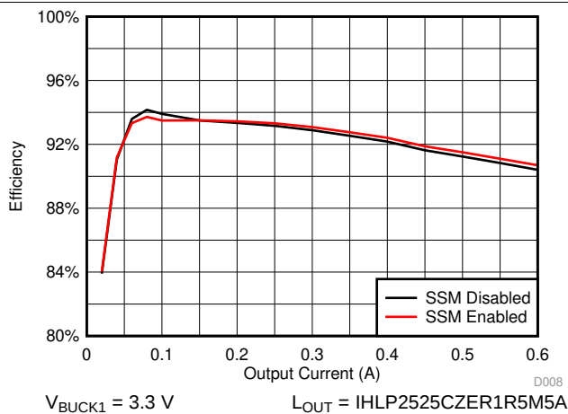
Figure 9-10. BOOST Efficiency
