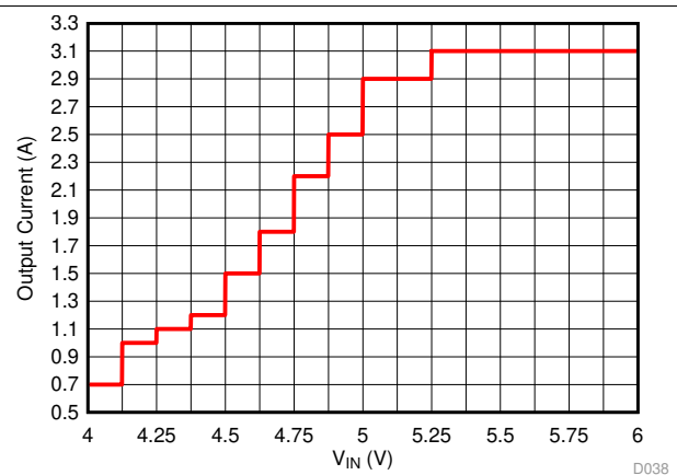
Figure 9-5. BUCK1 Output Current at Low V_{IN} Conditions
