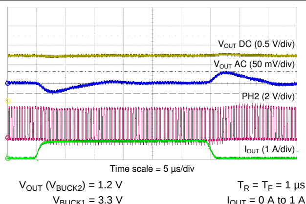
Figure 9-23. BUCK2 Load Transient
