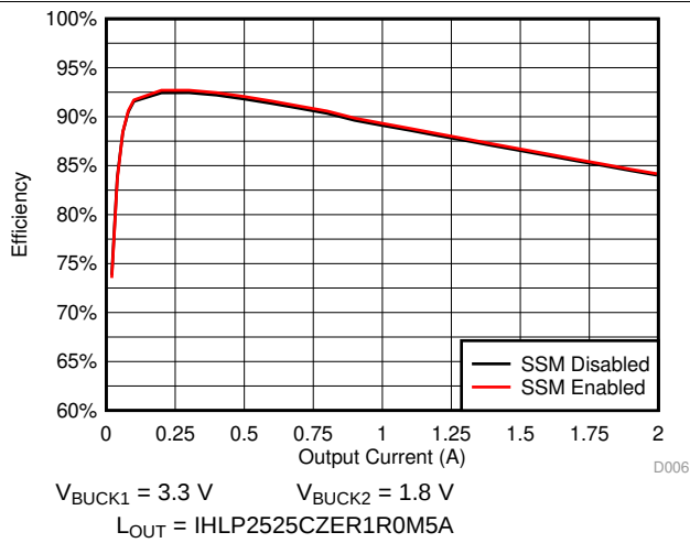
Figure 9-8. BUCK2 Efficiency
