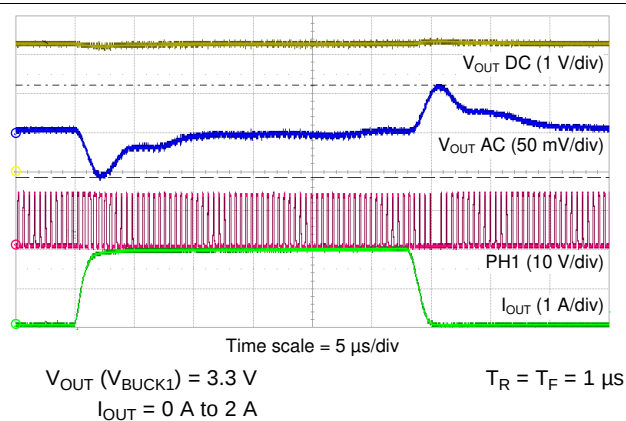
Figure 9-21. BUCK1 Load Transient
