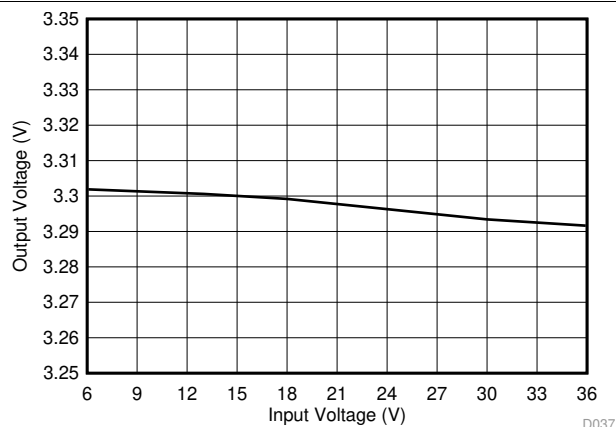
Figure 9-13. BUCK1 Line Regulation
