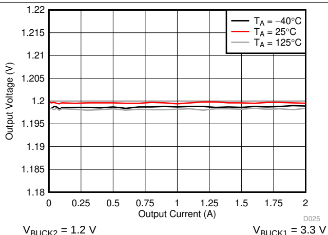
Figure 6-8. BUCK2 Output Voltage
