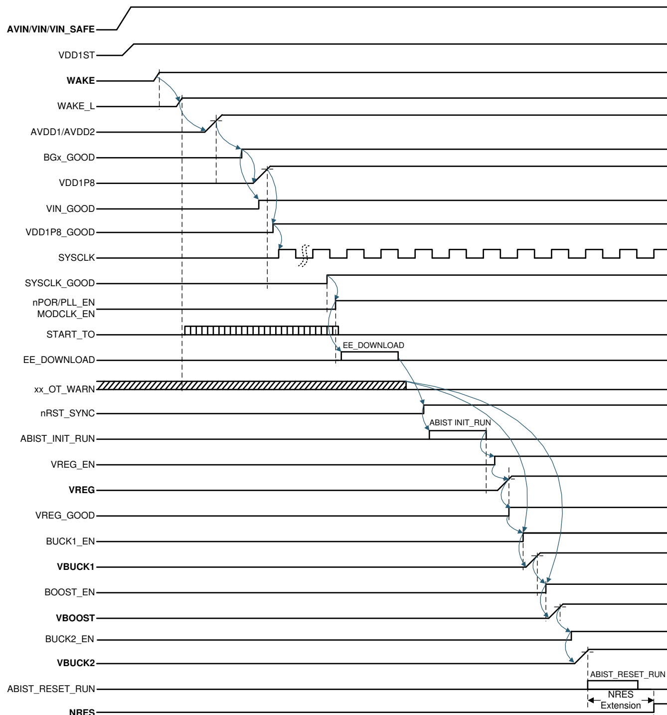
Figure 8-32. Power-Up Sequence Example
