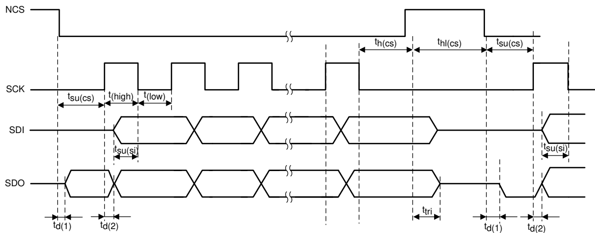
Figure 6-1. SPI Timing Parameters
