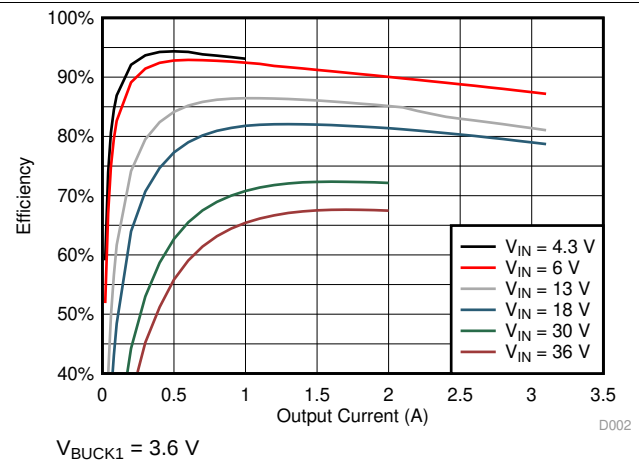
Figure 9-3. BUCK1 Efficiency
