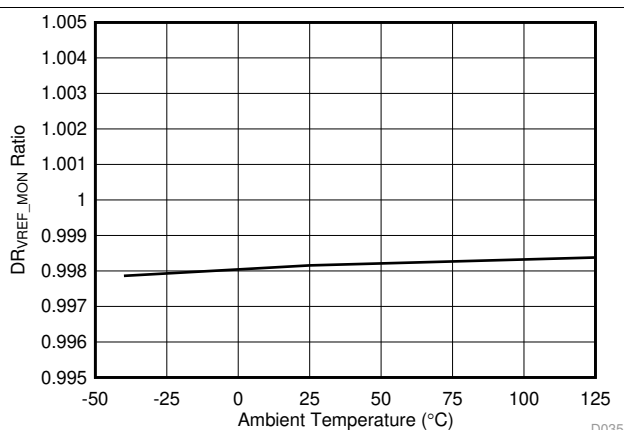
Figure 6-19. AMUX Output Division Ratio ( DRV_{REF\_MON} )
