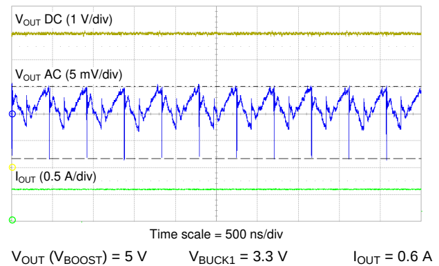
Figure 9-39. BOOST Output Voltage Ripple
