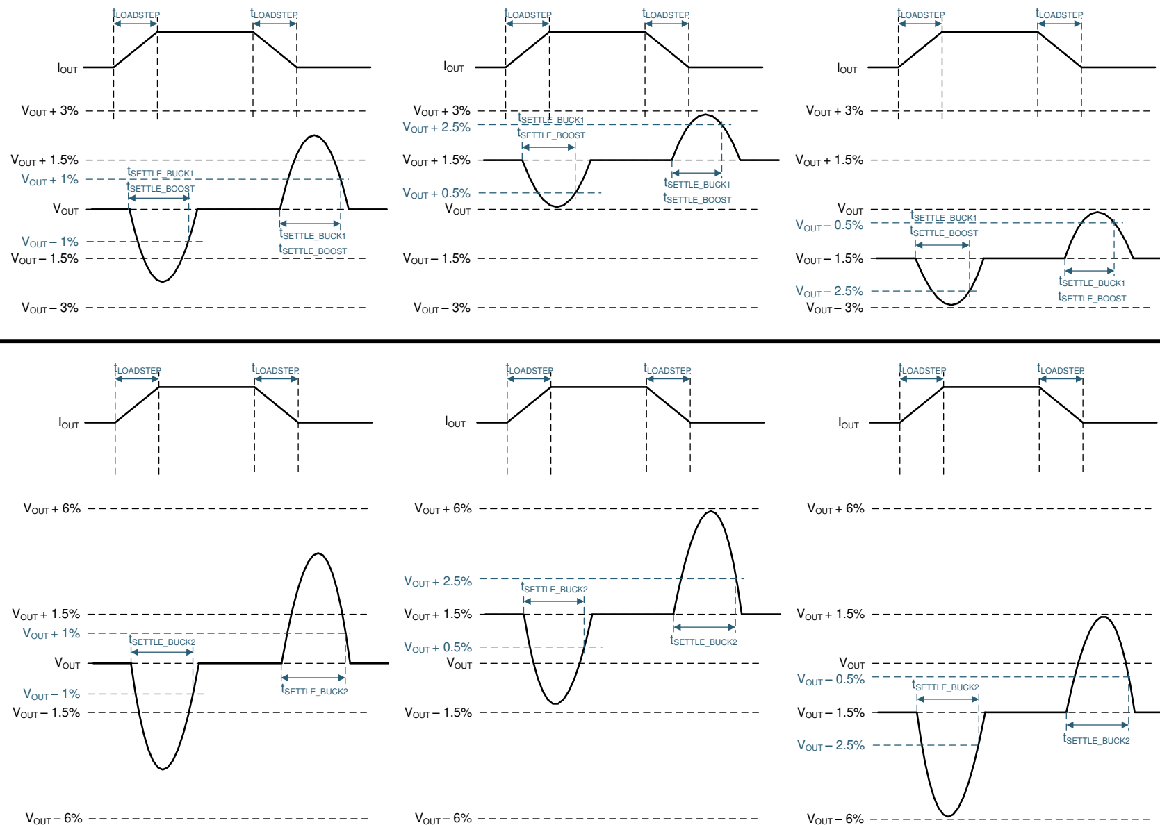
Figure 7-4. Regulator Load-Step Response
