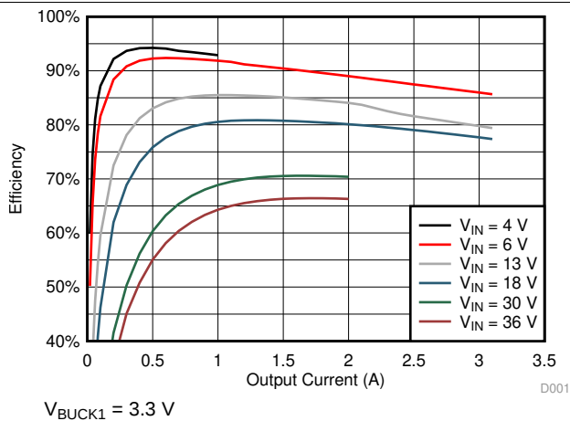
Figure 9-2. BUCK1 Efficiency
