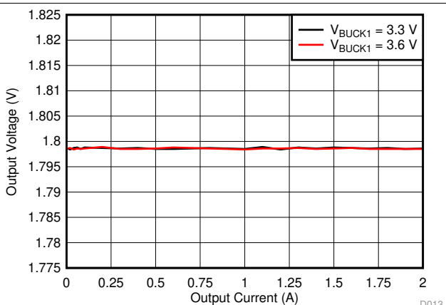
Figure 9-16. BUCK2 Load Regulation
