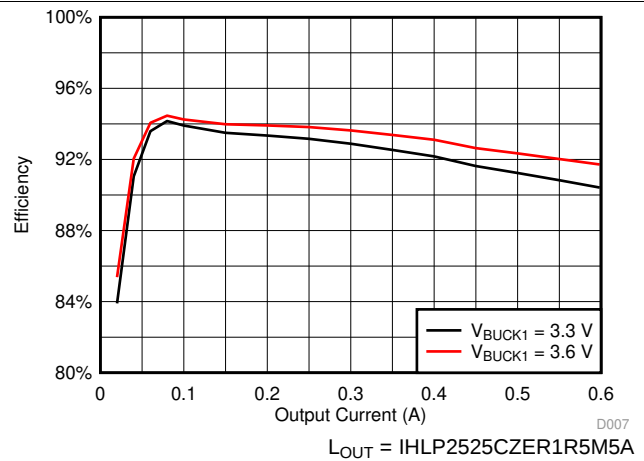
Figure 9-9. BOOST Efficiency
