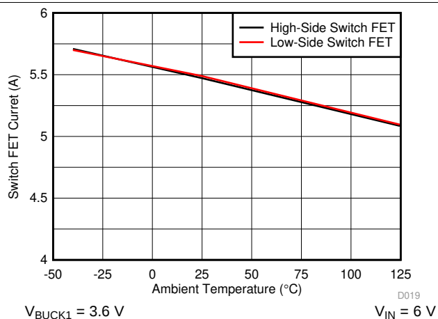
Figure 6-3. BUCK1 Current Limit ( I_{HS\_SCG\_ILIM\_BUCK1} and I_{LS\_SCG\_ILIM\_BUCK1} )
