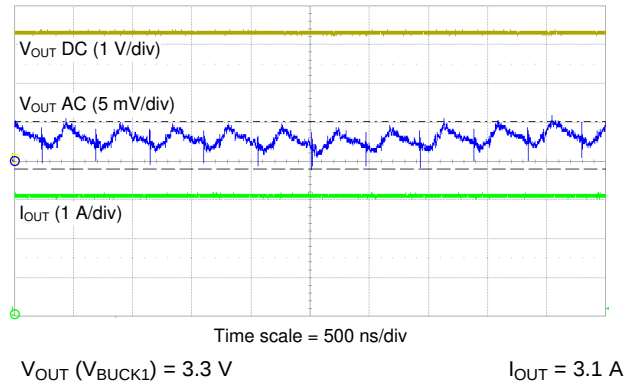
Figure 9-31. BUCK1 Output Voltage Ripple
