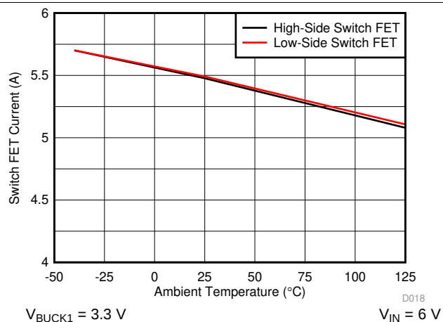
Figure 6-2. BUCK1 Current Limit ( I_{HS\_SCG\_ILIM\_BUCK1} and I_{LS\_SCG\_ILIM\_BUCK1} )
