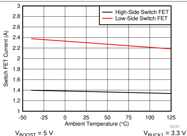
Figure 6-5. BOOST Current Limit ( I_{LS\_LIMIT\_BOOST} and I_{HS\_LIMIT\_BOOST} )
