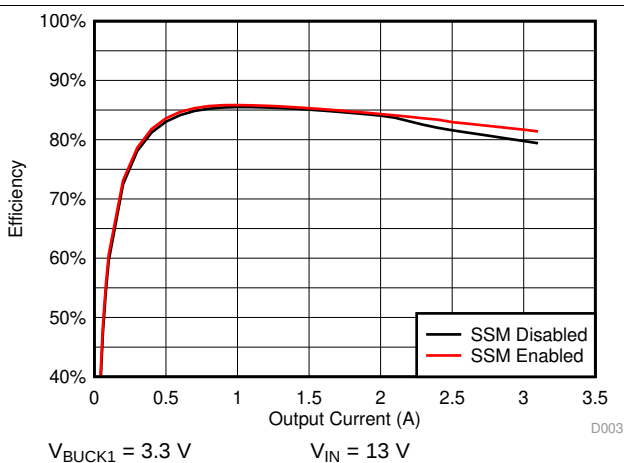
Figure 9-4. BUCK1 Efficiency
