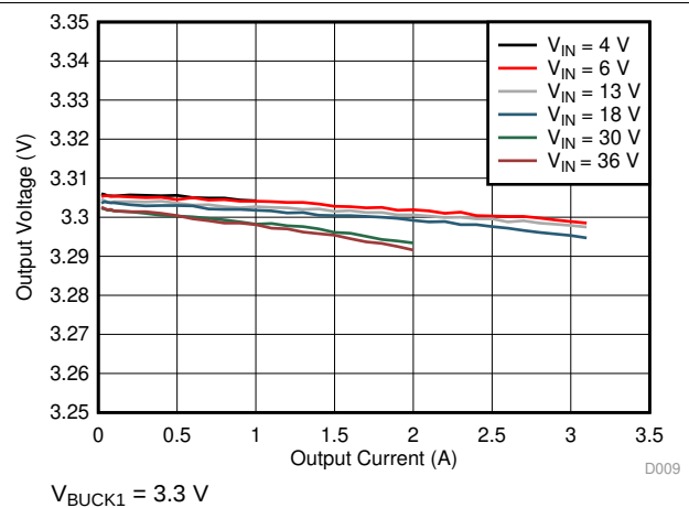
Figure 9-11. BUCK1 Load and Line Regulation
