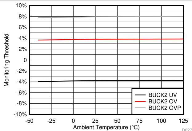
Figure 6-13. BUCK2 UV, OV, and OVP Threshold
