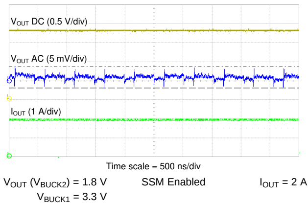
Figure 9-38. BUCK2 Output Voltage Ripple
