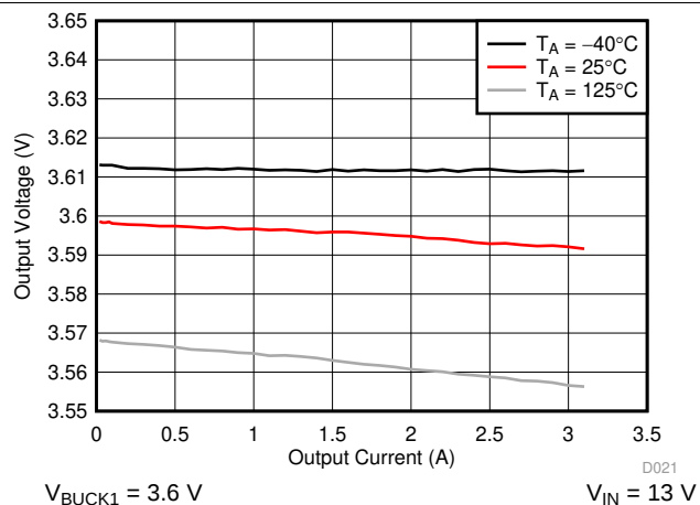
Figure 6-7. BUCK1 Output Voltage
