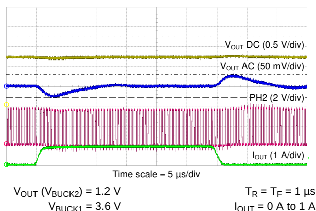
Figure 9-26. BUCK2 Load Transient
