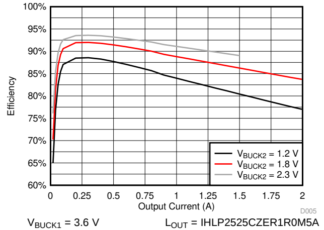
Figure 9-7. BUCK2 Efficiency
