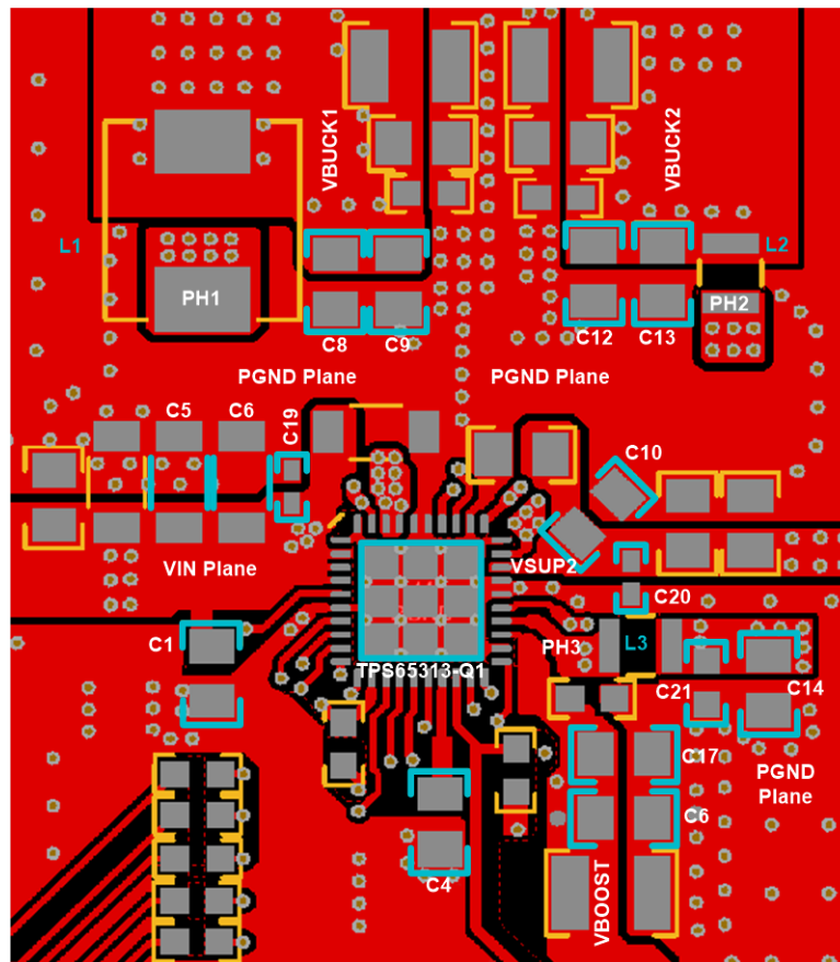
Figure 9-47. Layout Example
