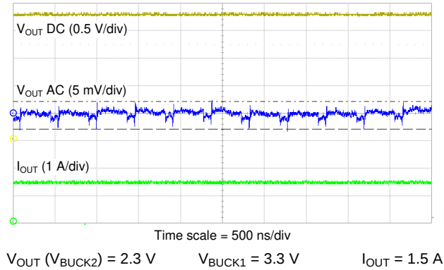
Figure 9-36. BUCK2 Output Voltage Ripple
