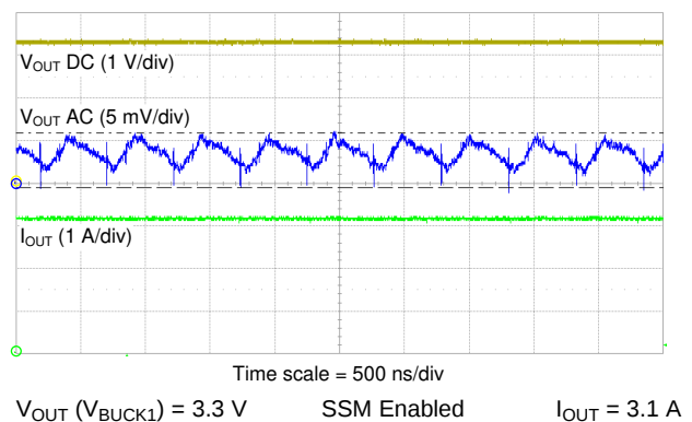
Figure 9-33. BUCK1 Output Voltage Ripple
