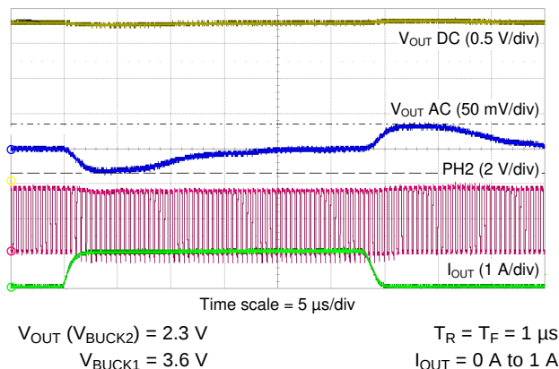
Figure 9-28. BUCK2 Load Transient
