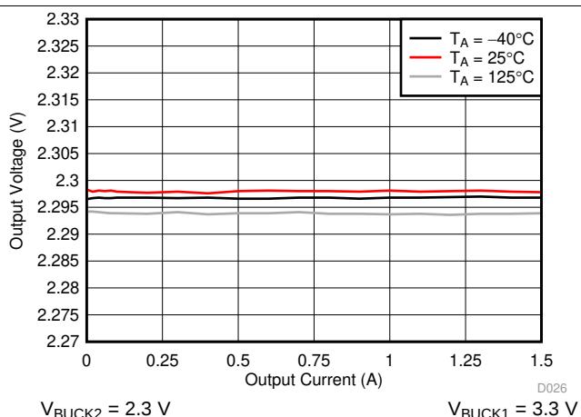
Figure 6-10. BUCK2 Output Voltage
