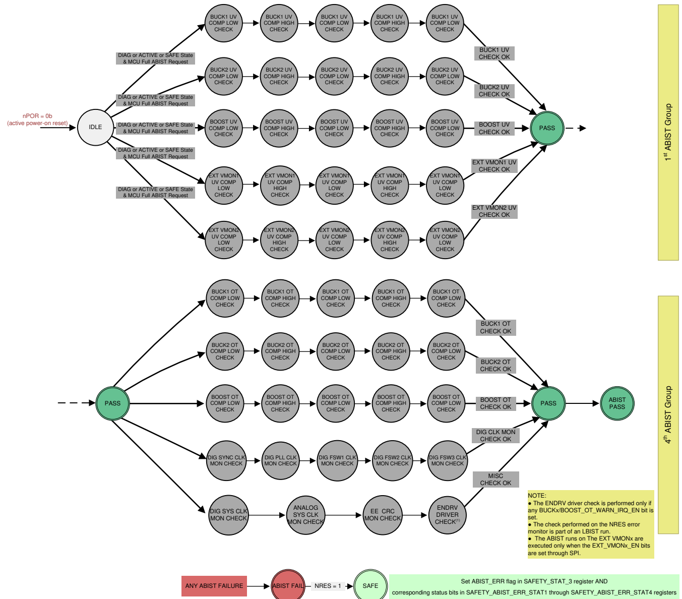
Figure 8-10. Partial ABIST Run When the Device is in the DIAGNOSTIC, ACTIVE, or SAFE State
