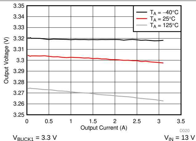
Figure 6-6. BUCK1 Output Voltage
