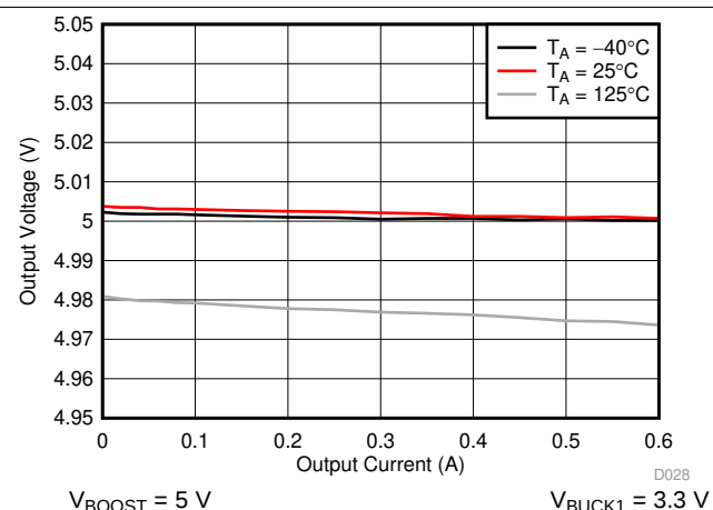
Figure 6-11. BOOST Output Voltage
