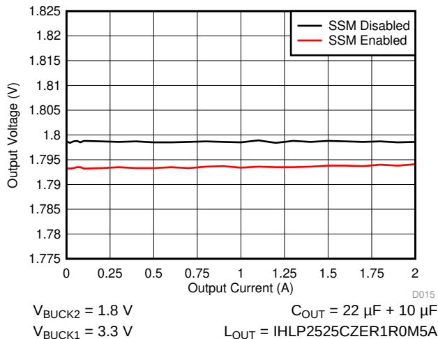
Figure 9-18. BUCK2 Load Regulation
