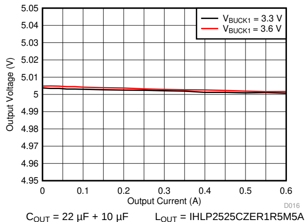
Figure 9-19. BOOST Load and Line Regulation
