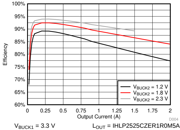
Figure 9-6. BUCK2 Efficiency
