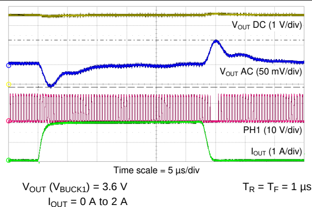
Figure 9-22. BUCK1 Load Transient
