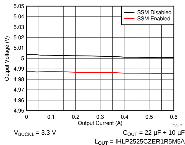
Figure 9-20. BOOST Load Regulation
