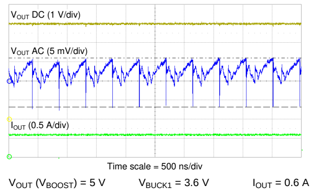
Figure 9-40. BOOST Output Voltage Ripple
