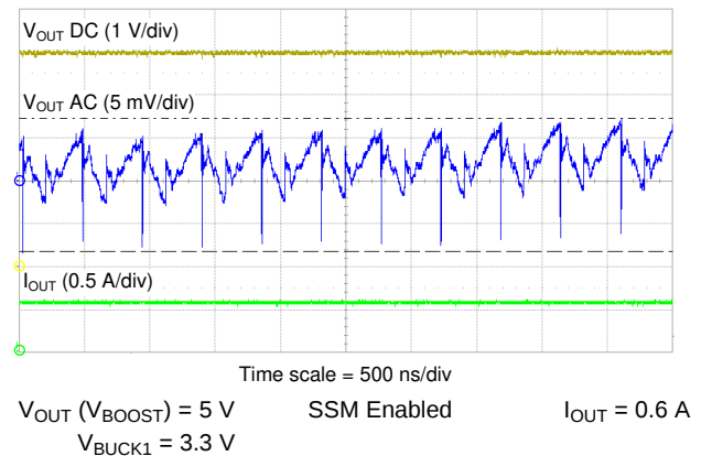
Figure 9-41. BOOST Output Voltage Ripple
