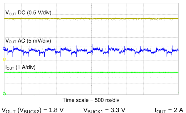
Figure 9-35. BUCK2 Output Voltage Ripple
