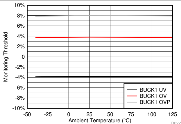
Figure 6-12. BUCK1 UV, OV, and OVP Threshold
