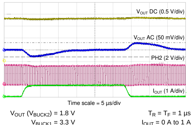
Figure 9-24. BUCK2 Load Transient
