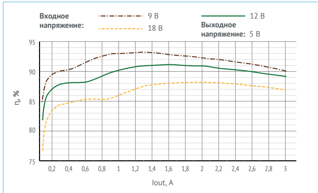
Рис. 11. V_{IN} = 9...18 \text{ В} ; V_{OUT} = 5 \text{ В} .
