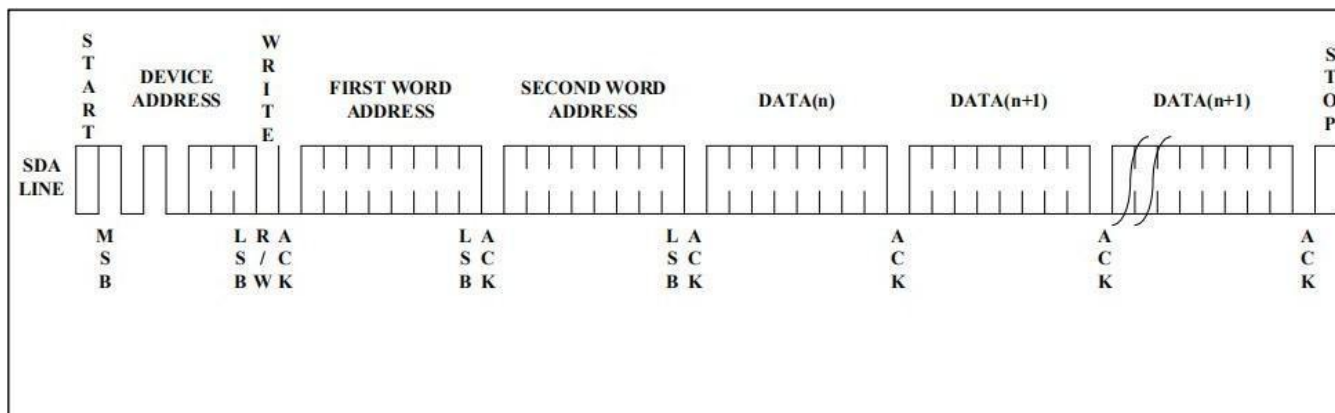
Figure 7. Page Write
