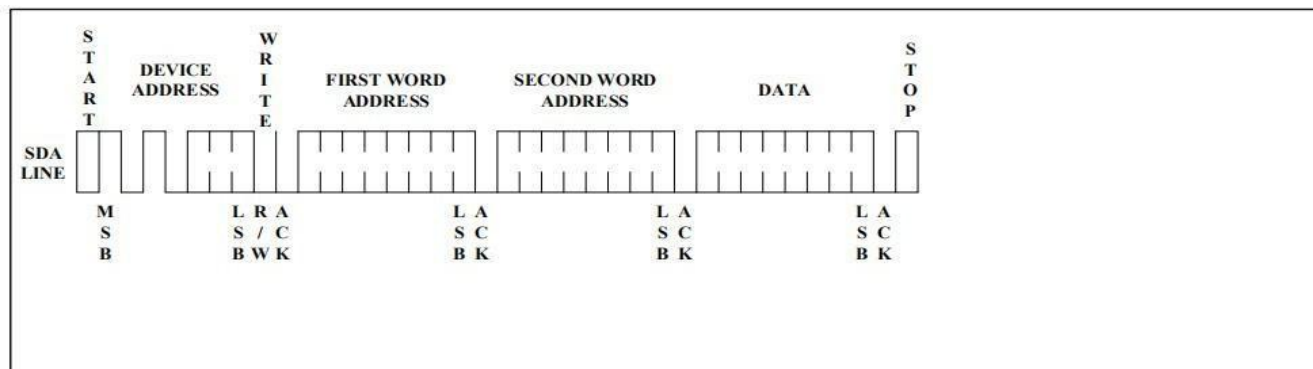
Figure 6. Byte Write
